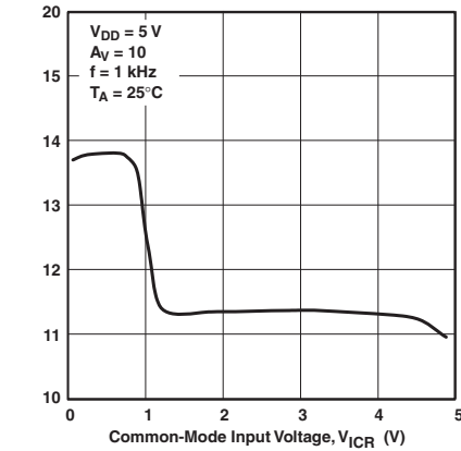
Figure 31. Equivalent Input Noise Voltage vs Common-Mode Input Voltage
