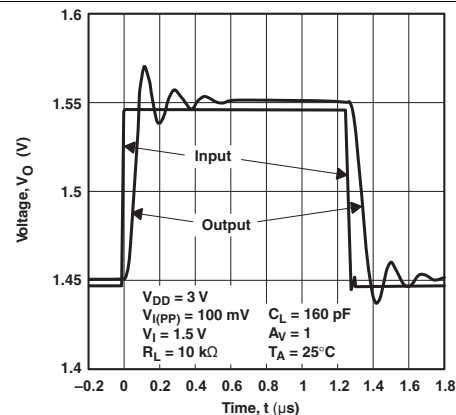
Figure 42. Small Signal Follower, V_{DD} = 3 V
