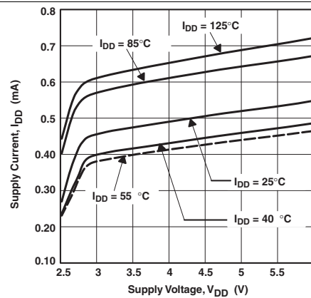
Figure 20. Supply Current vs Supply Voltage
