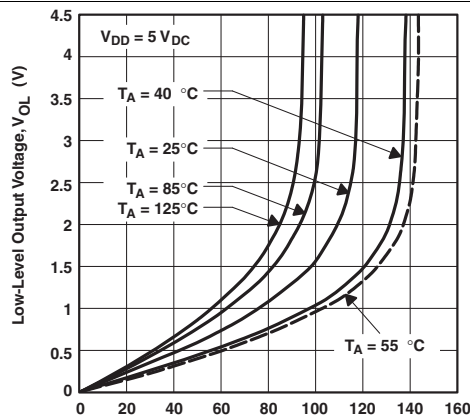
Figure 8. Low-level Output Voltage vs Low-level Output Current, V_{DD} = 5 V_{DC}
