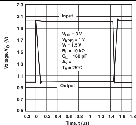
Figure 44. Inverting Large Signal, V_{DD} = 3\text{ V}
